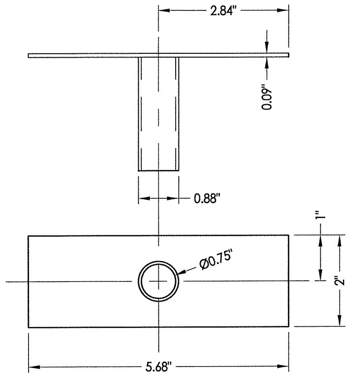
9 TUBE ANCHOR
